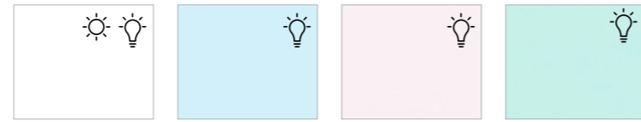
Opal S302 [12/6 mm] Δ E5 Sapphire S303 [12 mm] Ruby S304 [12 mm] Emerald S305 [12 mm]
